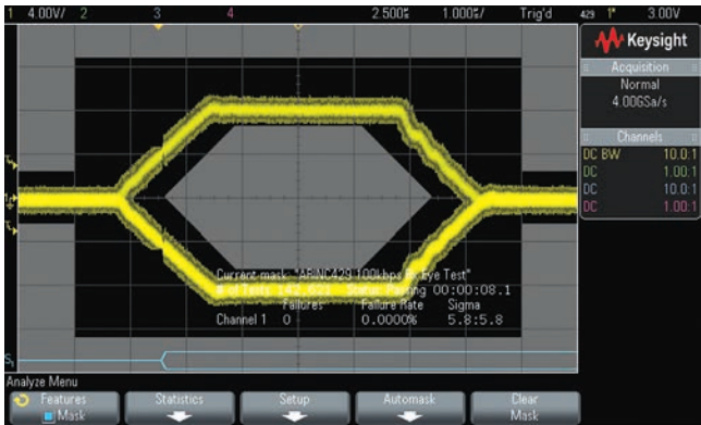
Figure 9. ARINC 429 100 kbps eye-diagram mask test.
