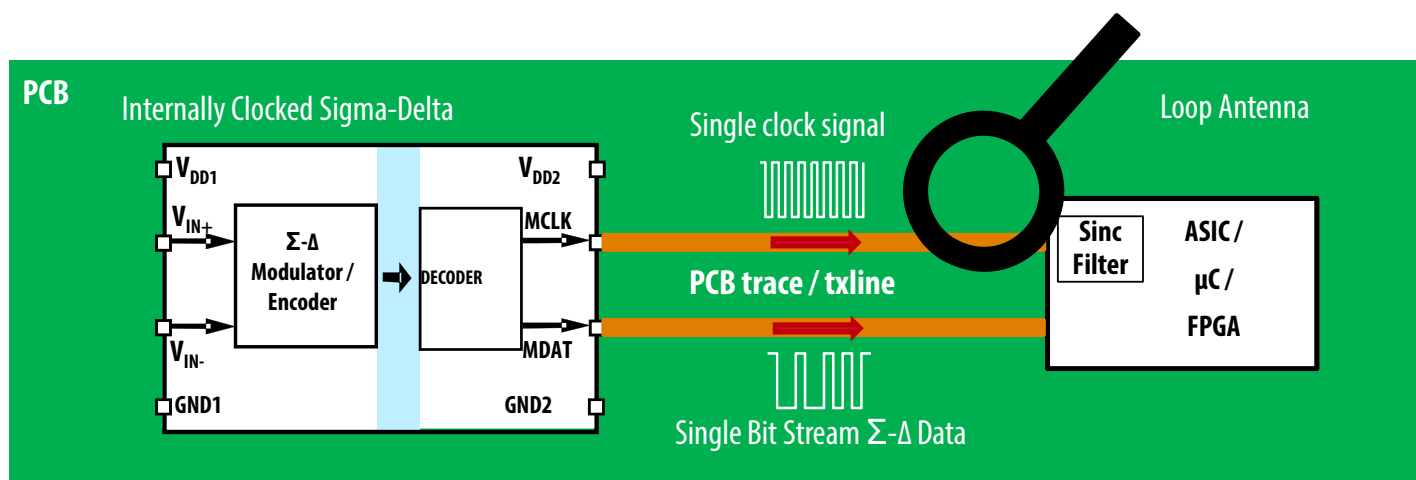
Figure 3 Receiver Loop Antenna Placed on the PCB Trace Where Single Clock Signal From an Internally Clocked Sigma-Delta Modulator is Routed to the Digital Filter
