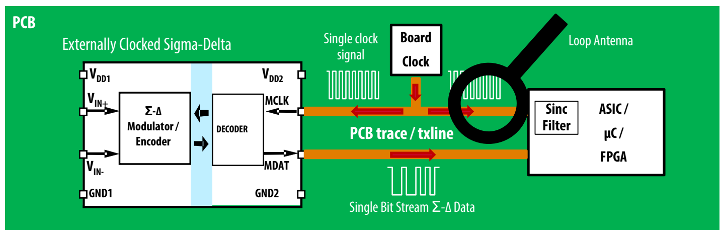
Figure 1 A Receiver Loop Antenna is Placed on the PCB Trace Where a Single Clock Signal is Routed to an Externally Clocked Sigma-Delta Modulator and Digital Filter
